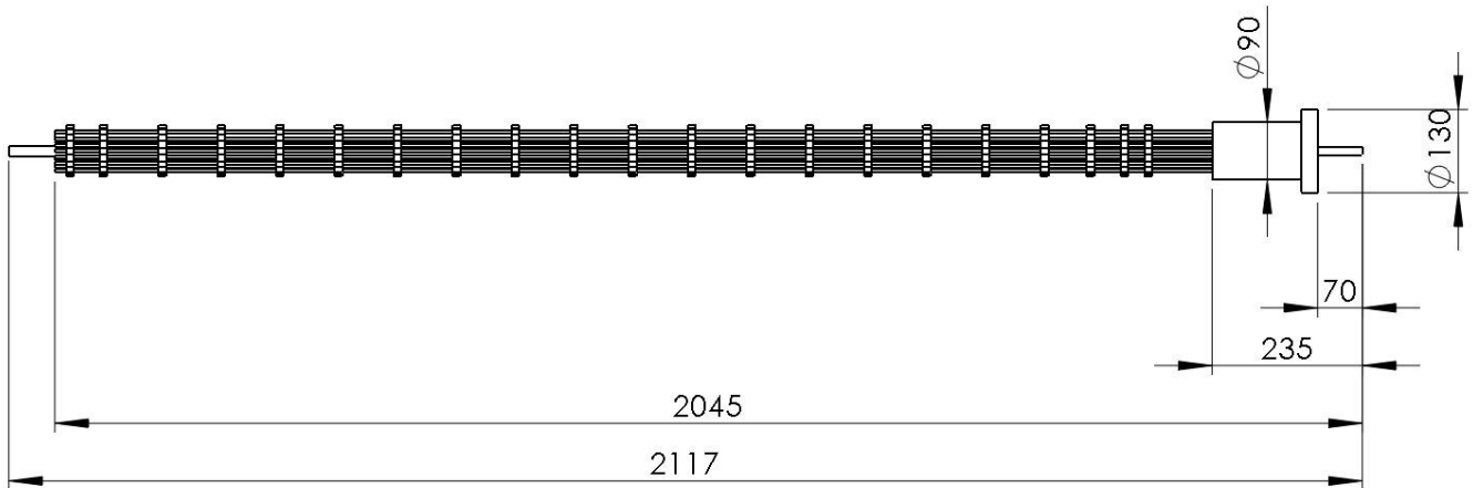
Abmessungen Tubothal Heizelement 500 / Dimensions Tubothal heating element 500
